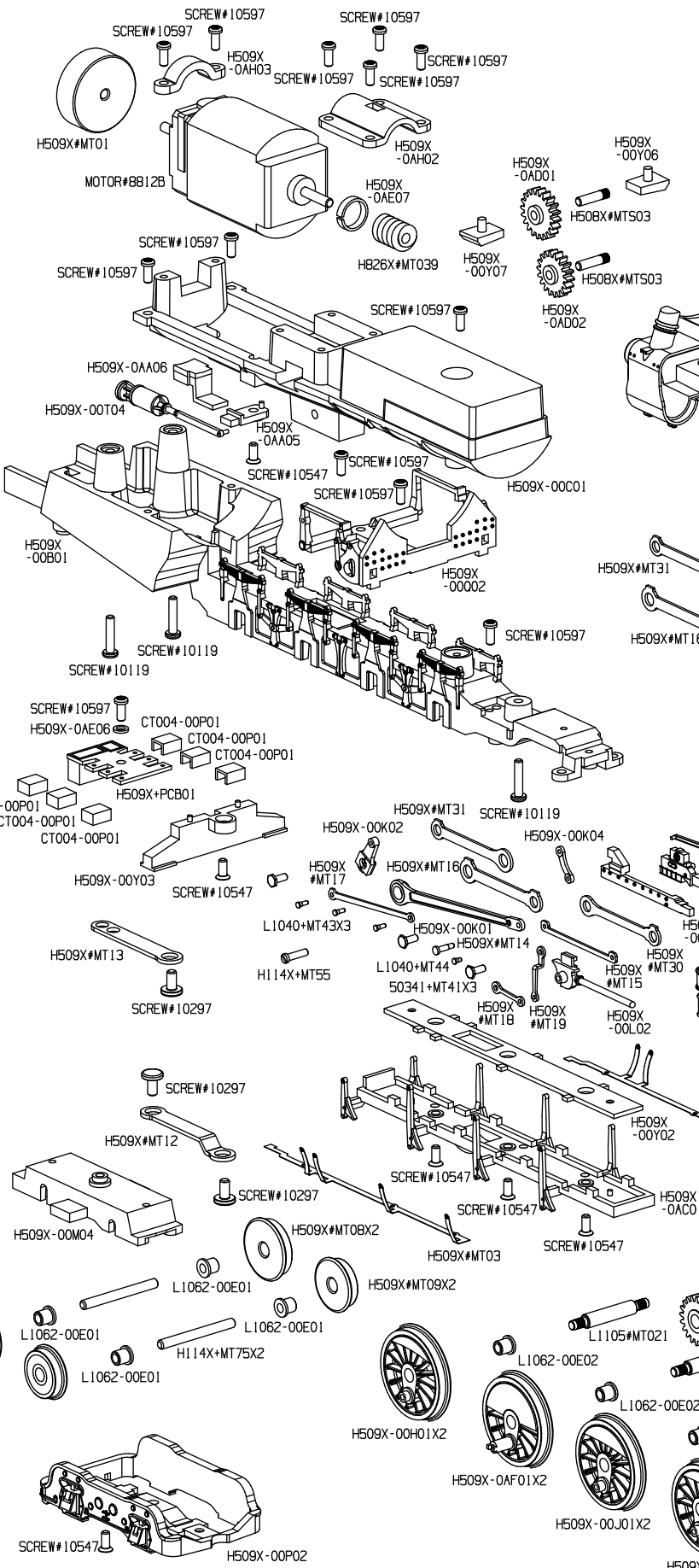
COMMON LOCO CHASSIS
