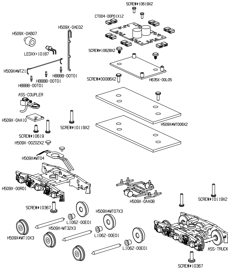
TENDER BODY-A
