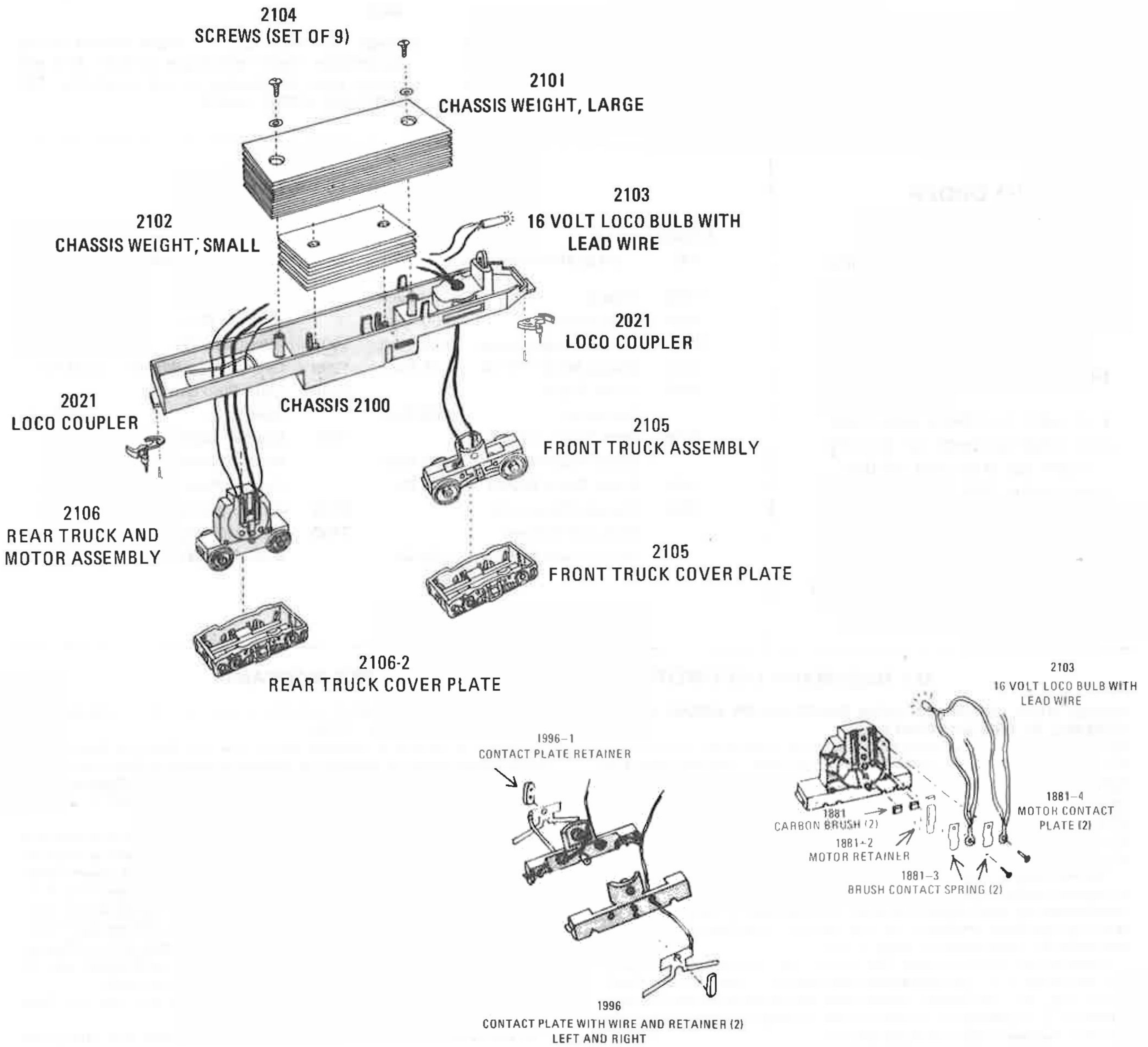
CHASSIS ASSEMBLY
