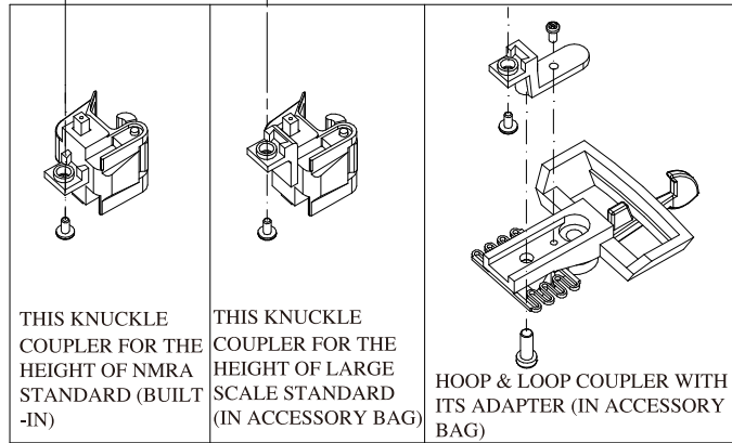
HIGH COUPLER
